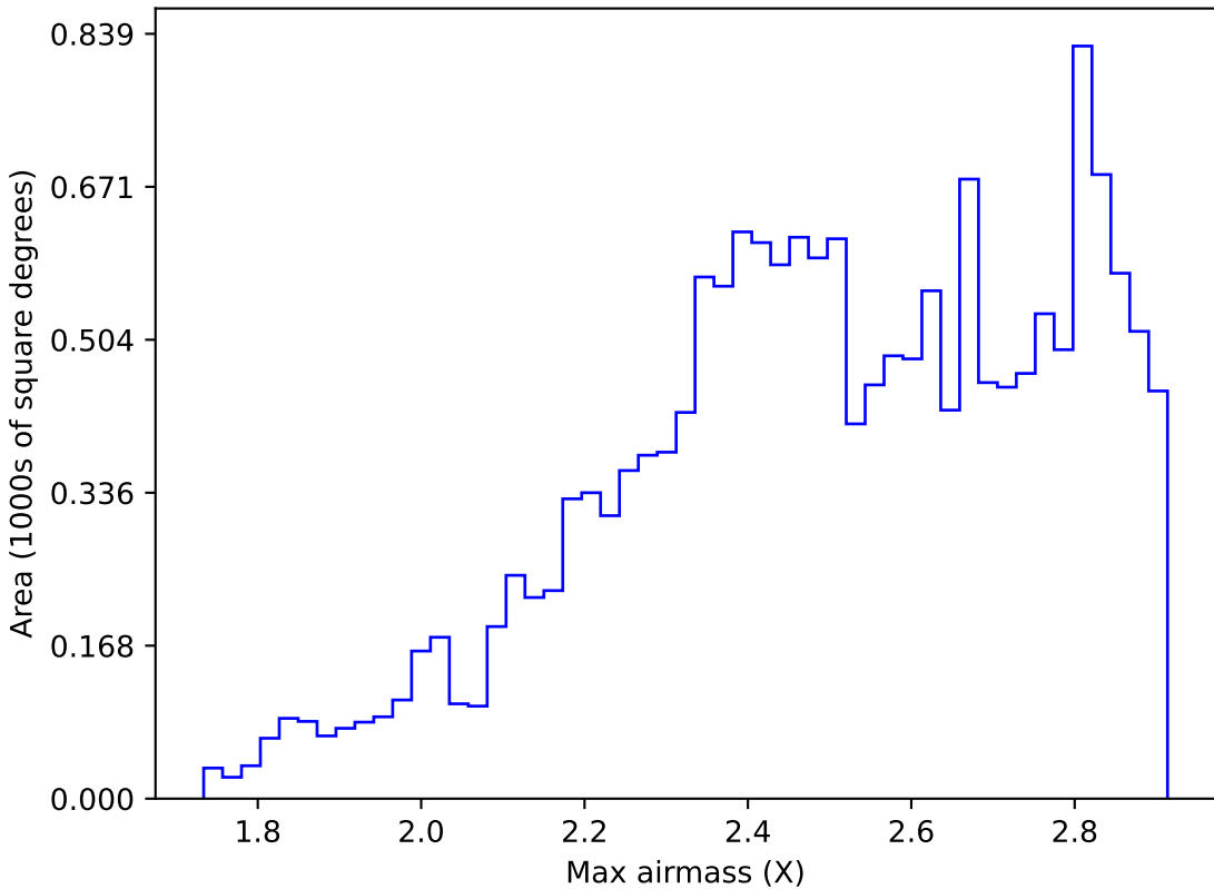
internal_u_expt30_nscale0.9v3.4_10yrs WFD z band: Max airmass
