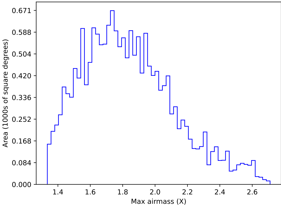
internal_u_expt30_nscale0.9v3.4_10yrs WFD u band: Max airmass
