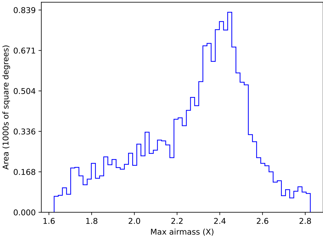
internal_u_expt30_nscale0.9v3.4_10yrs WFD r band: Max airmass
