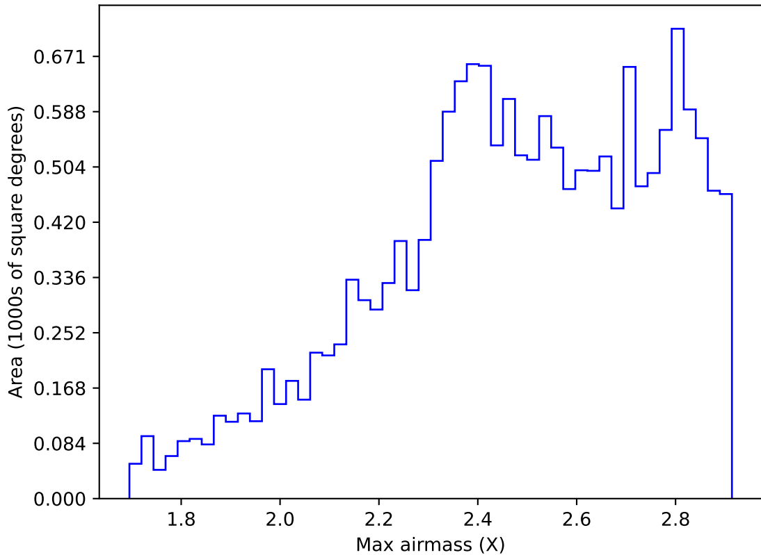
internal_u_expt30_nscale0.9v3.4_10yrs WFD i band: Max airmass
