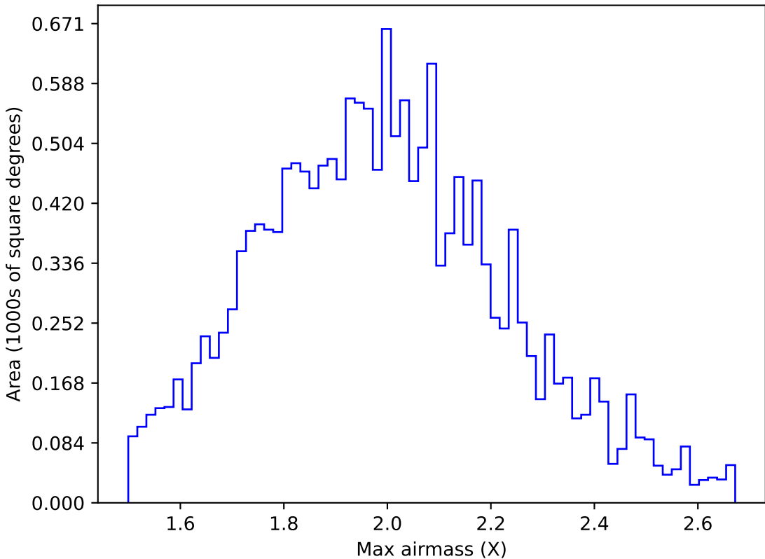
internal_u_expt30_nscale0.9v3.4_10yrs WFD g band: Max airmass
