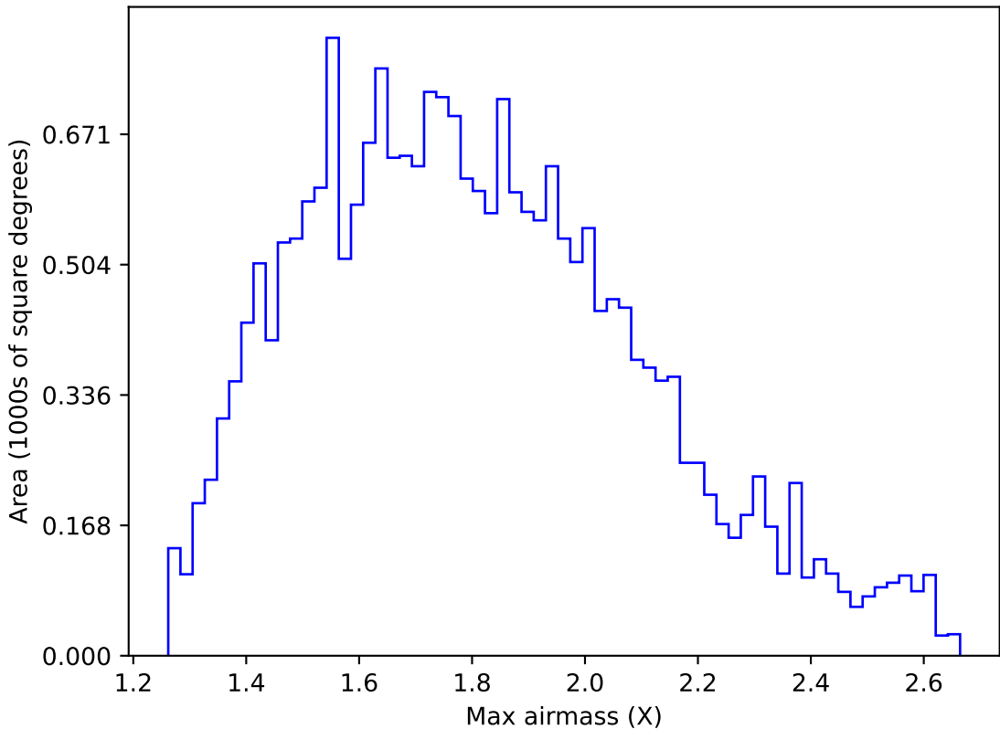
internal_u_expt30_nscale0.9v3.4_10yrs All sky u band: Max airmass
