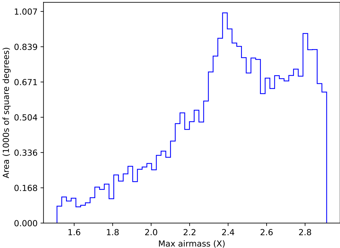
internal_u_expt30_nscale0.9v3.4_10yrs All sky i band: Max airmass
