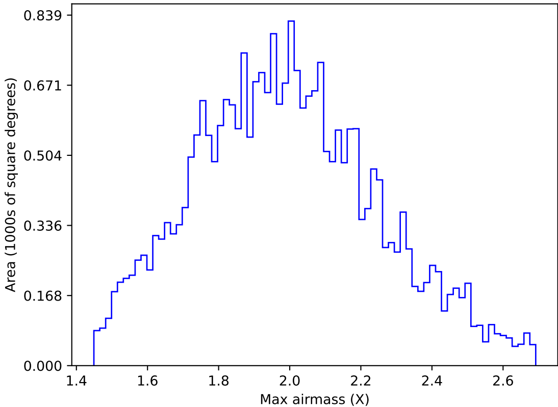
internal_u_expt30_nscale0.9v3.4_10yrs All sky g band: Max airmass
