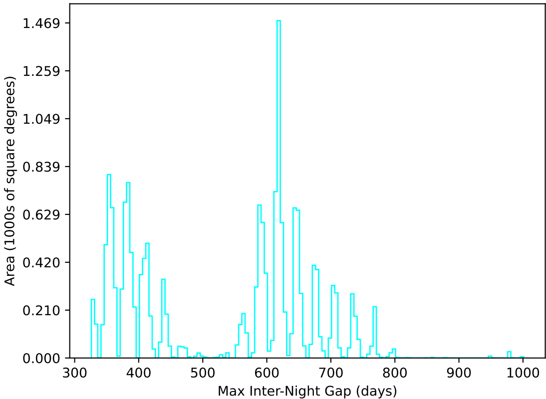
internal_u_expt30_nscale0.9v3.4_10yrs WFD u band: Max Inter-Night Gap
