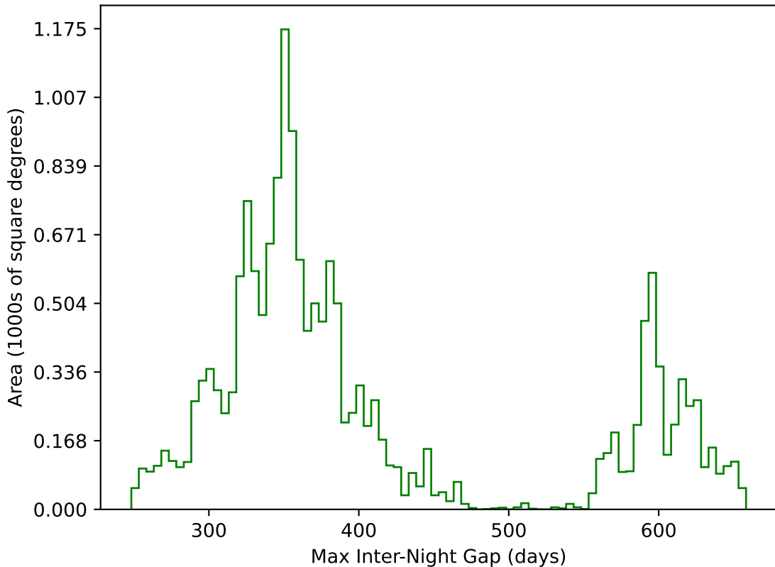
internal_u_expt30_nscale0.9v3.4_10yrs WFD g band: Max Inter-Night Gap
