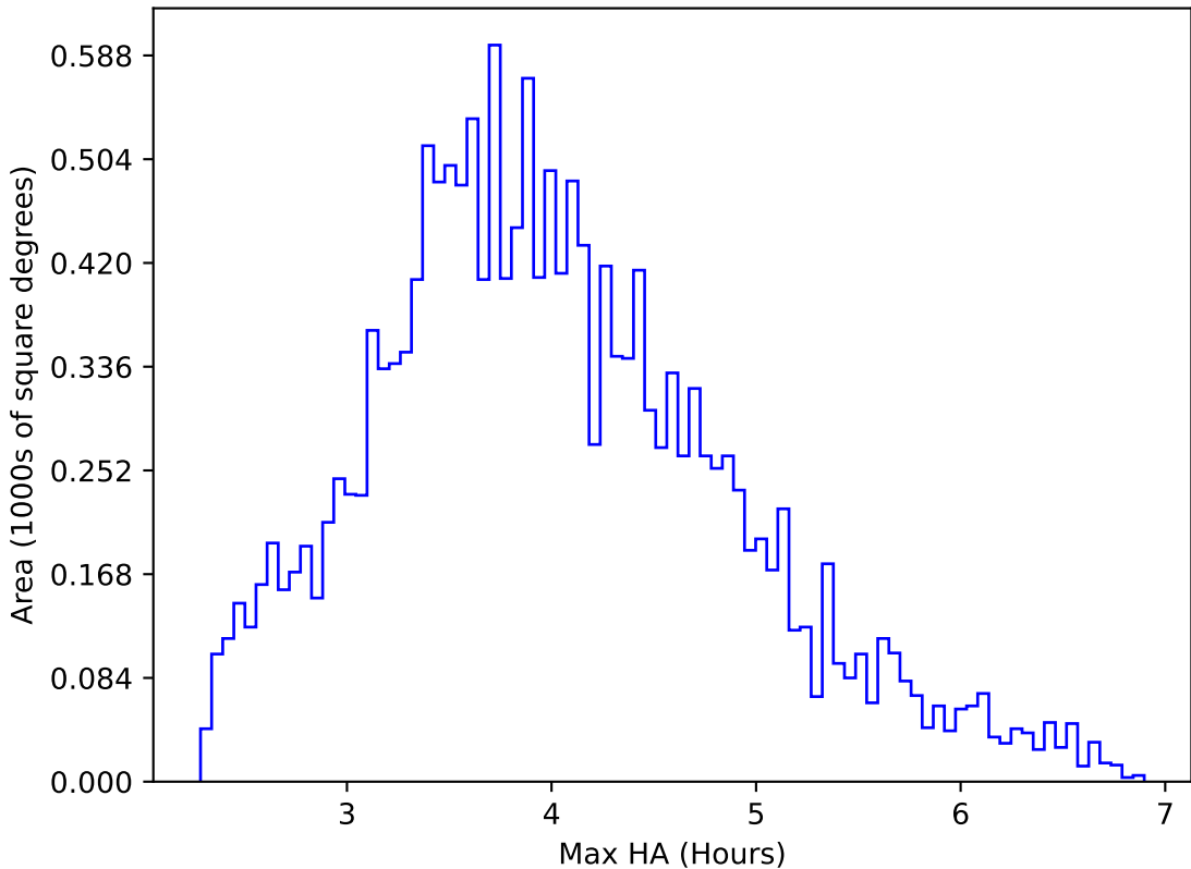
internal_u_expt30_nscale0.9v3.4_10yrs WFD g band: Max HA
