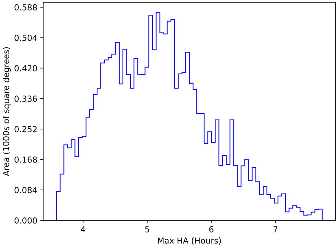
internal_u_expt30_nscale0.9v3.4_10yrs WFD all bands: Max HA
