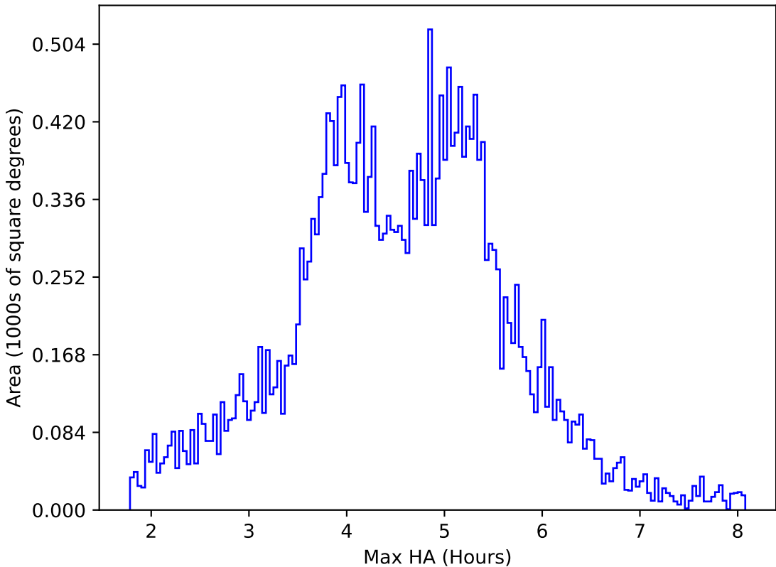
internal_u_expt30_nscale0.9v3.4_10yrs All sky z band: Max HA
