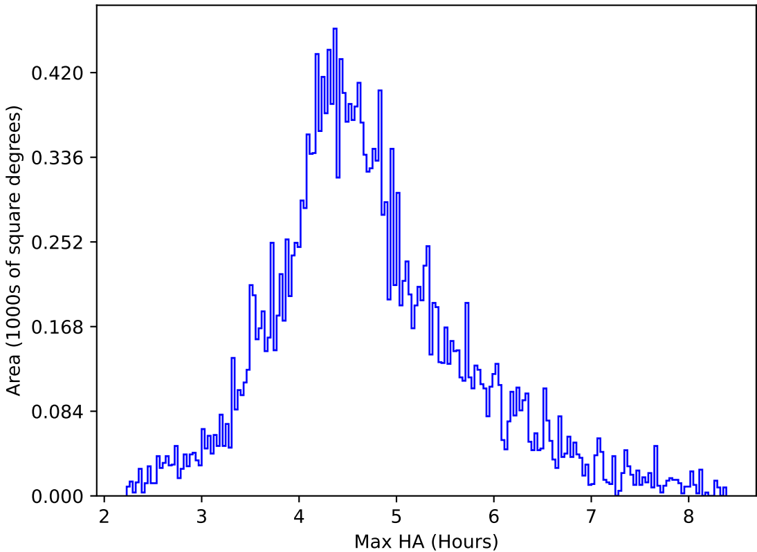
internal_u_expt30_nscale0.9v3.4_10yrs All sky y band: Max HA
