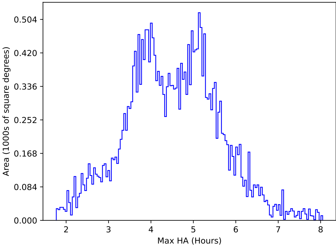
internal_u_expt30_nscale0.9v3.4_10yrs All sky i band: Max HA
