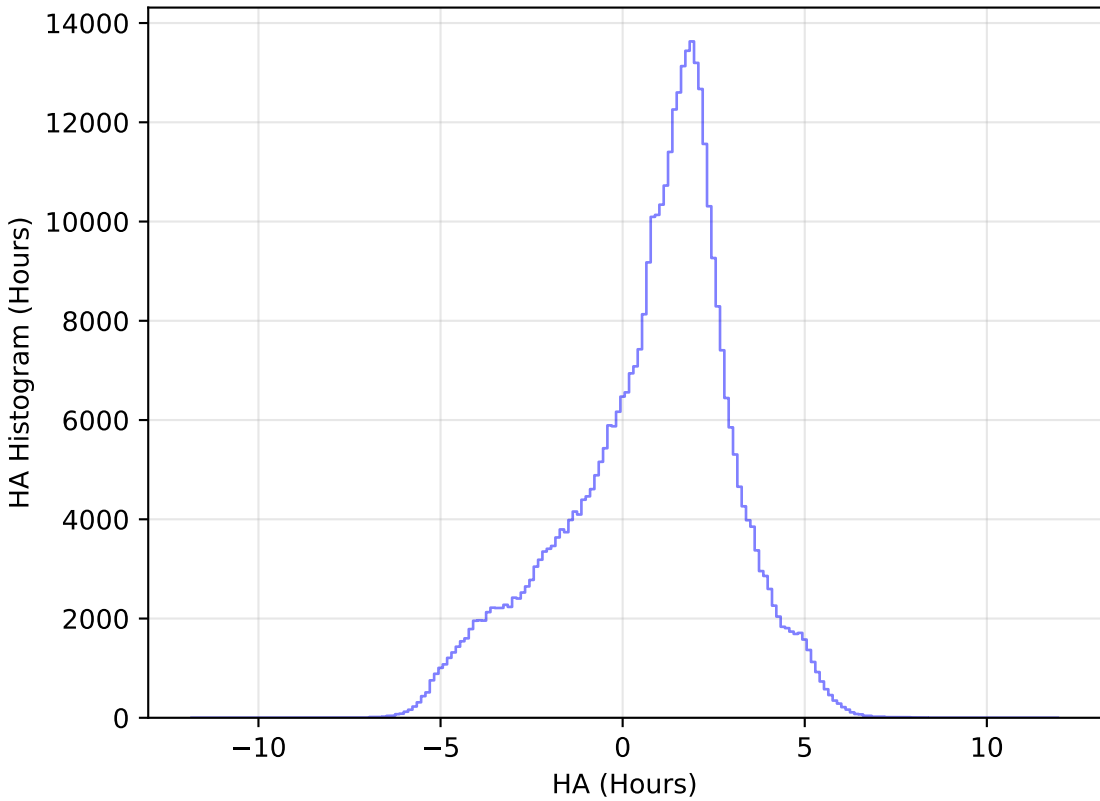
internal_u_expt30_nscale0.9v3.4_10yrs WFD z band: HA Histogram
