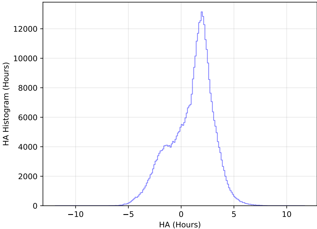
internal_u_expt30_nscale0.9v3.4_10yrs WFD y band: HA Histogram
