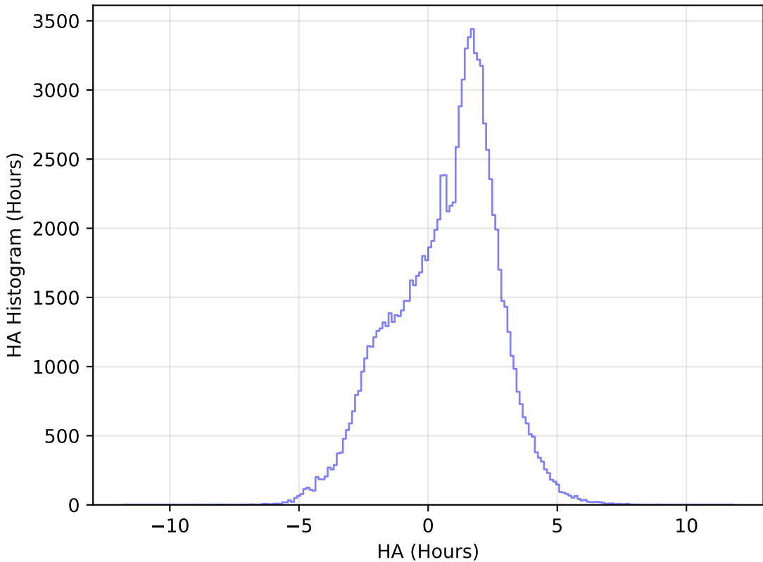
internal_u_expt30_nscale0.9v3.4_10yrs WFD u band: HA Histogram
