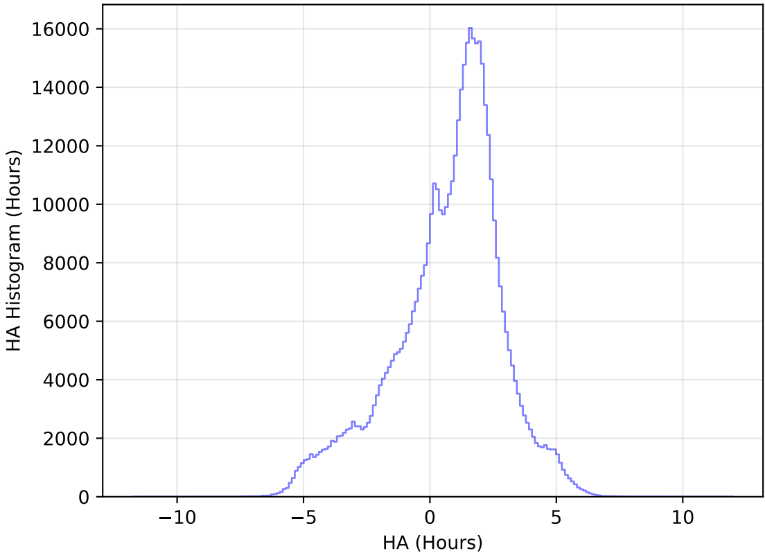
internal_u_expt30_nscale0.9v3.4_10yrs WFD i band: HA Histogram
