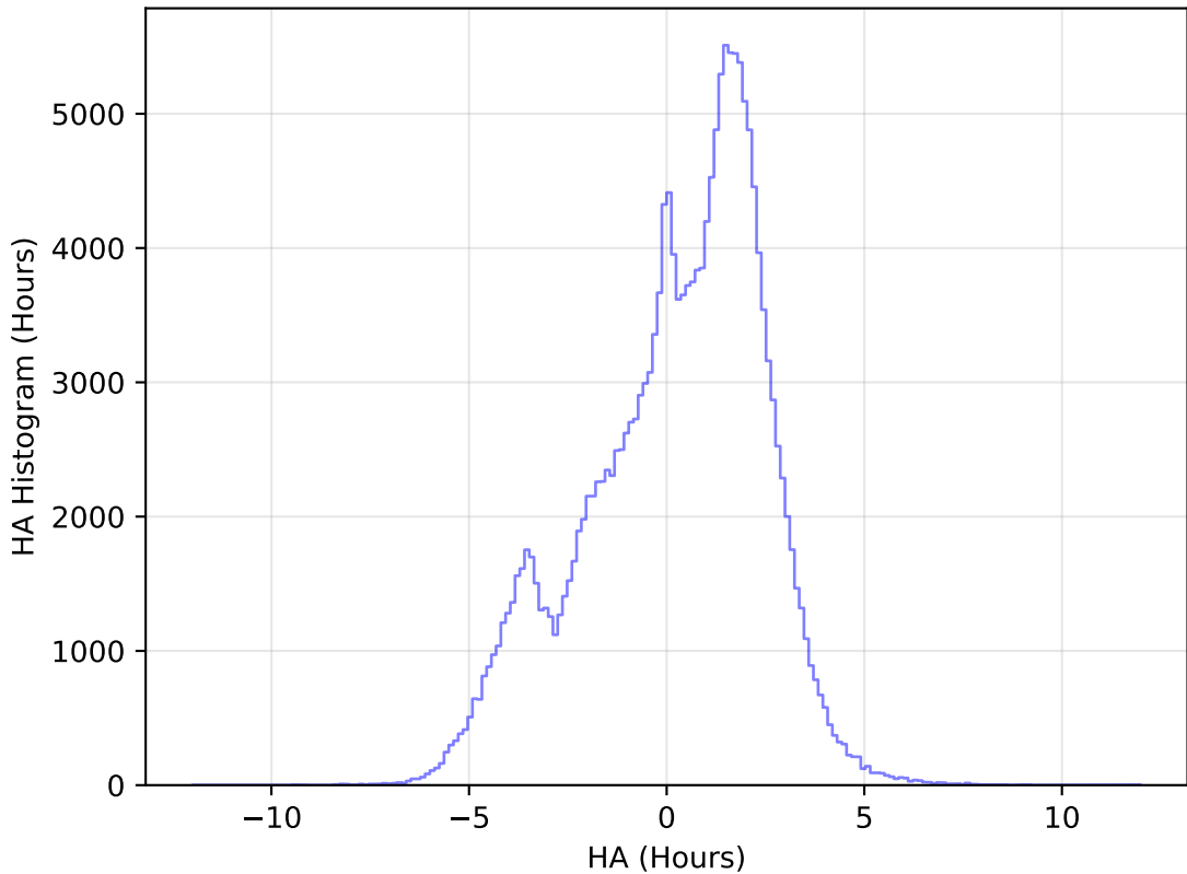
internal_u_expt30_nscale0.9v3.4_10yrs WFD g band: HA Histogram
