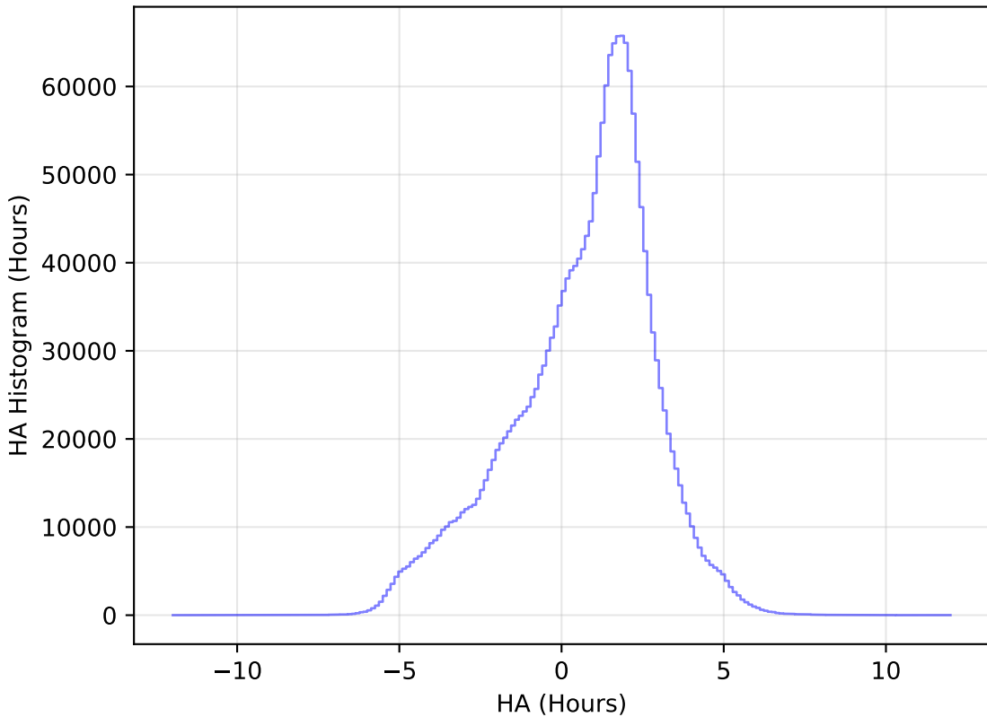
internal_u_expt30_nscale0.9v3.4_10yrs WFD all bands: HA Histogram
