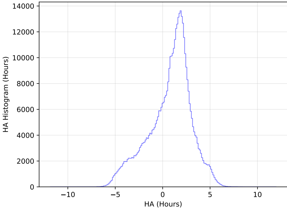
internal_u_expt30_nscale0.9v3.4_10yrs All sky z band: HA Histogram
