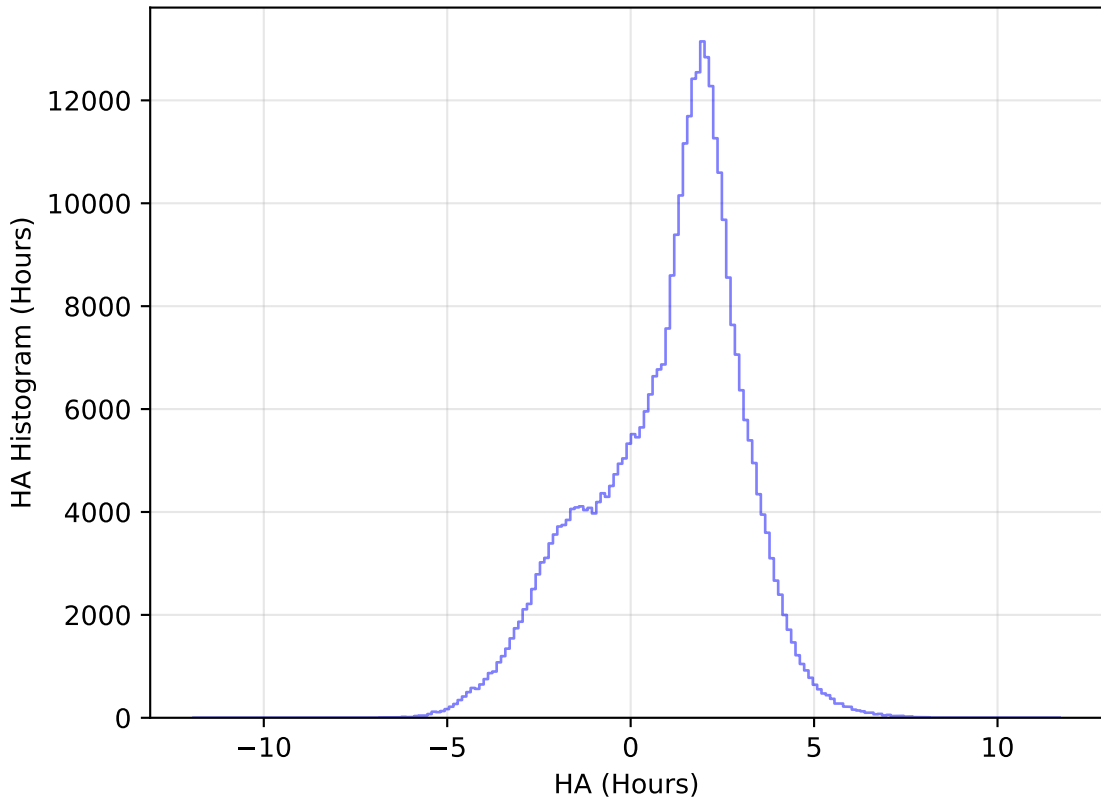
internal_u_expt30_nscale0.9v3.4_10yrs All sky y band: HA Histogram
