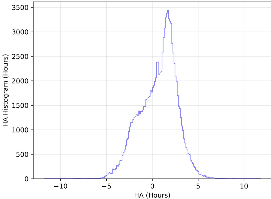
internal_u_expt30_nscale0.9v3.4_10yrs All sky u band: HA Histogram
