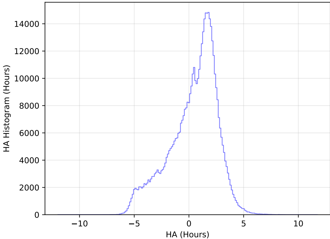
internal_u_expt30_nscale0.9v3.4_10yrs All sky r band: HA Histogram
