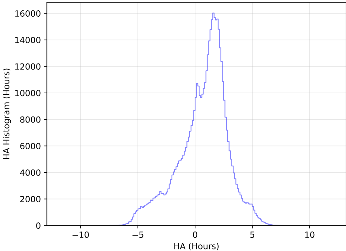
internal_u_expt30_nscale0.9v3.4_10yrs All sky i band: HA Histogram
