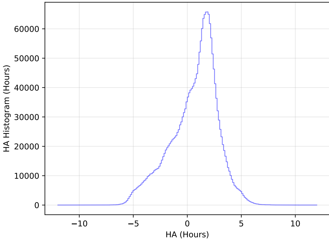
internal_u_expt30_nscale0.9v3.4_10yrs All sky all bands: HA Histogram
