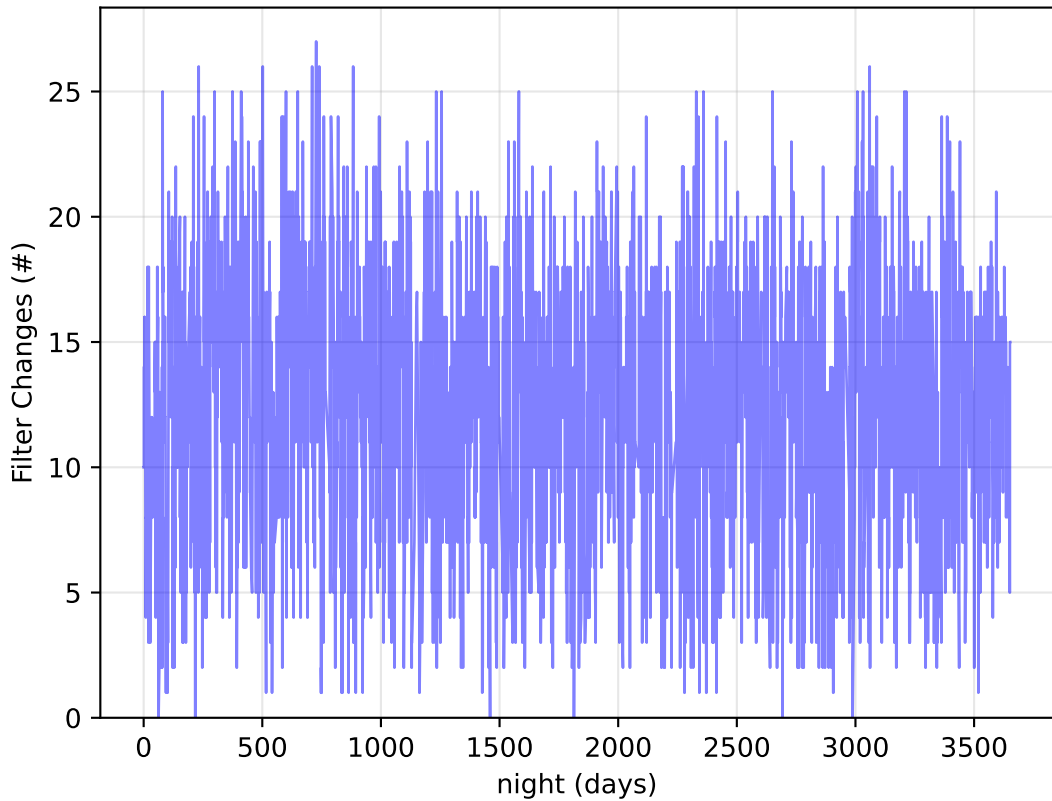
internal_u_expt30_nscale0.9v3.4_10yrs Per Night: Filter Changes
