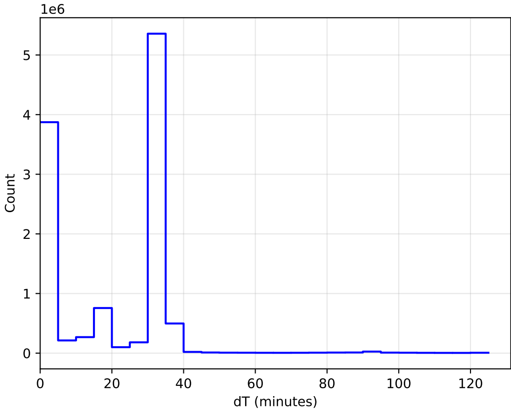
internal_u_expt30_nscale0.9v3.4_10yrs WFD: DeltaT Histogram
