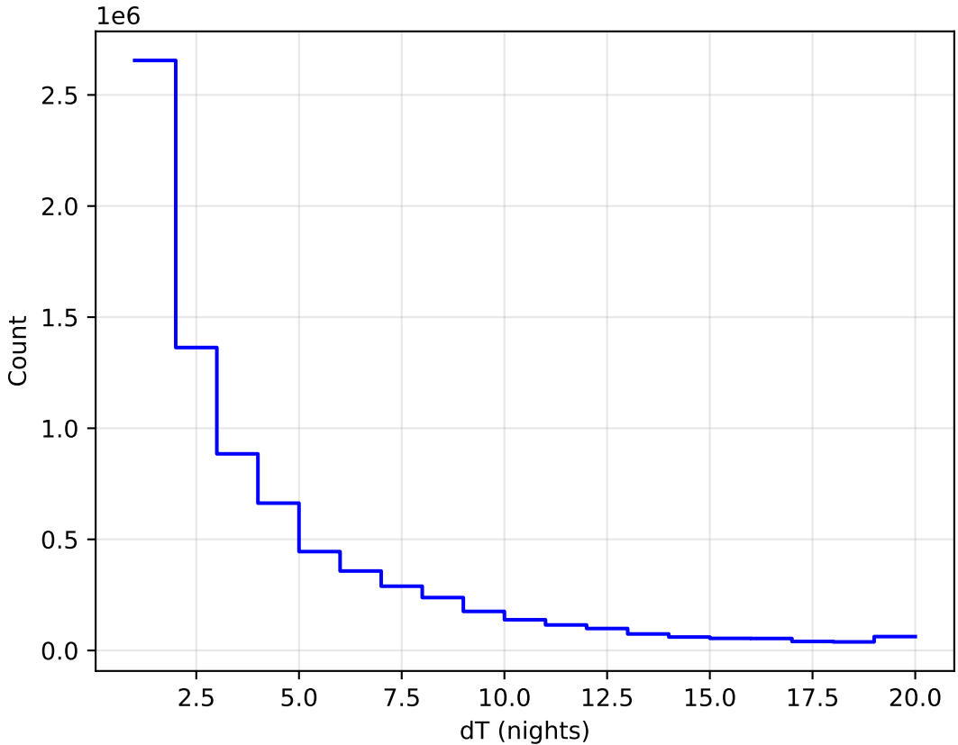
internal_u_expt30_nscale0.9v3.4_10yrs WFD all bands: DeltaNight Histogram
