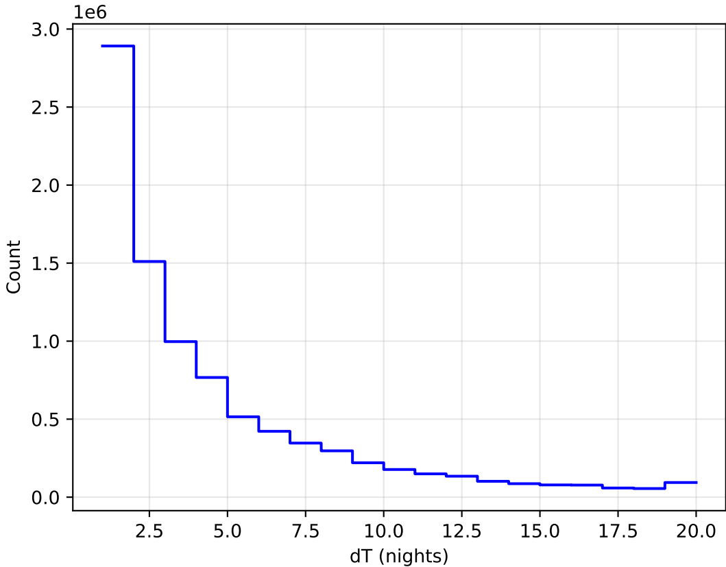
internal_u_expt30_nscale0.9v3.4_10yrs All sky all bands: DeltaNight Histogram
