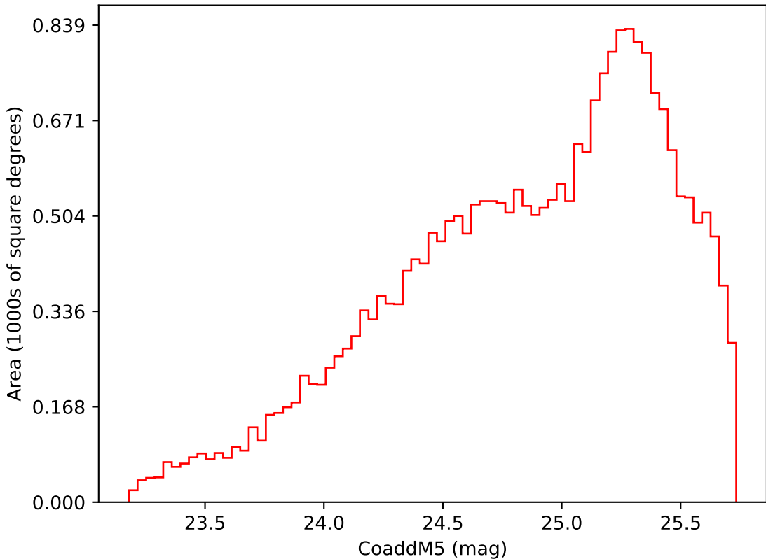
internal_u_expt30_nscale0.9v3.4_10yrs Yr 3-4 i band: CoaddM5
