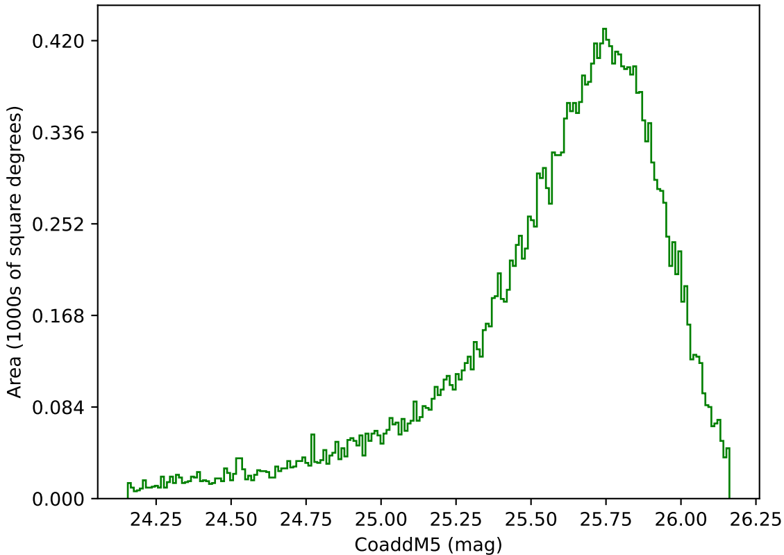
internal_u_expt30_nscale0.9v3.4_10yrs Yr 1 g band: CoaddM5
