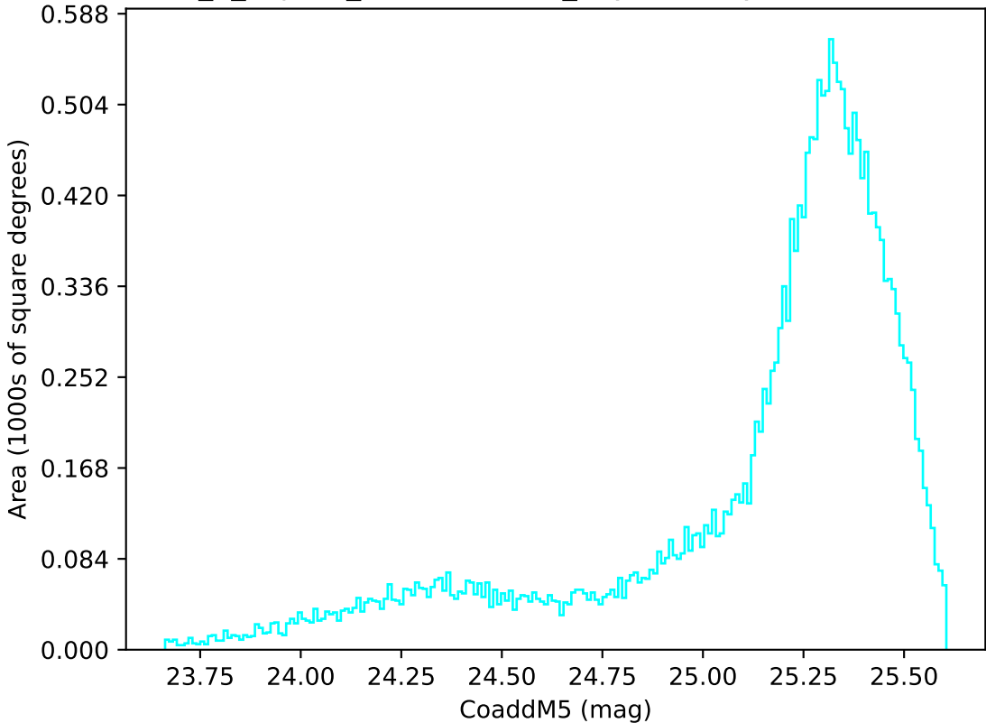
internal_u_expt30_nscale0.9v3.4_10yrs All sky u band: CoaddM5
