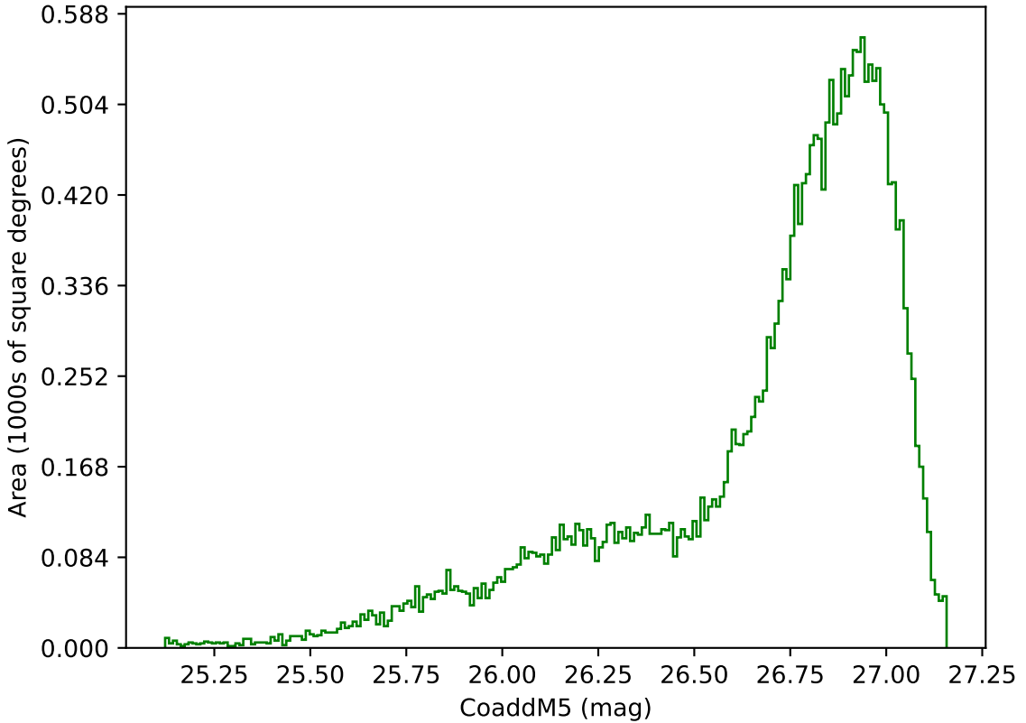
internal_u_expt30_nscale0.9v3.4_10yrs All sky g band: CoaddM5
