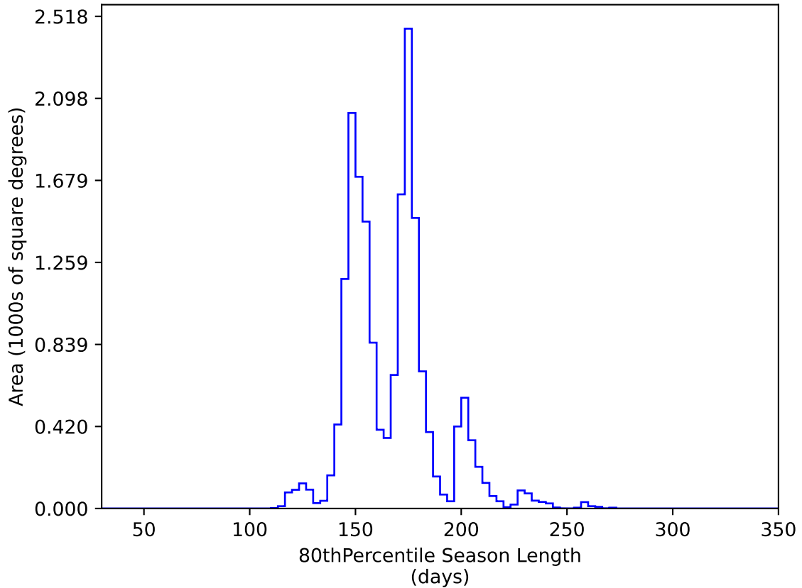
internal_u_expt30_nscale0.9v3.4_10yrs WFD y band: 80thPercentile Season Length
