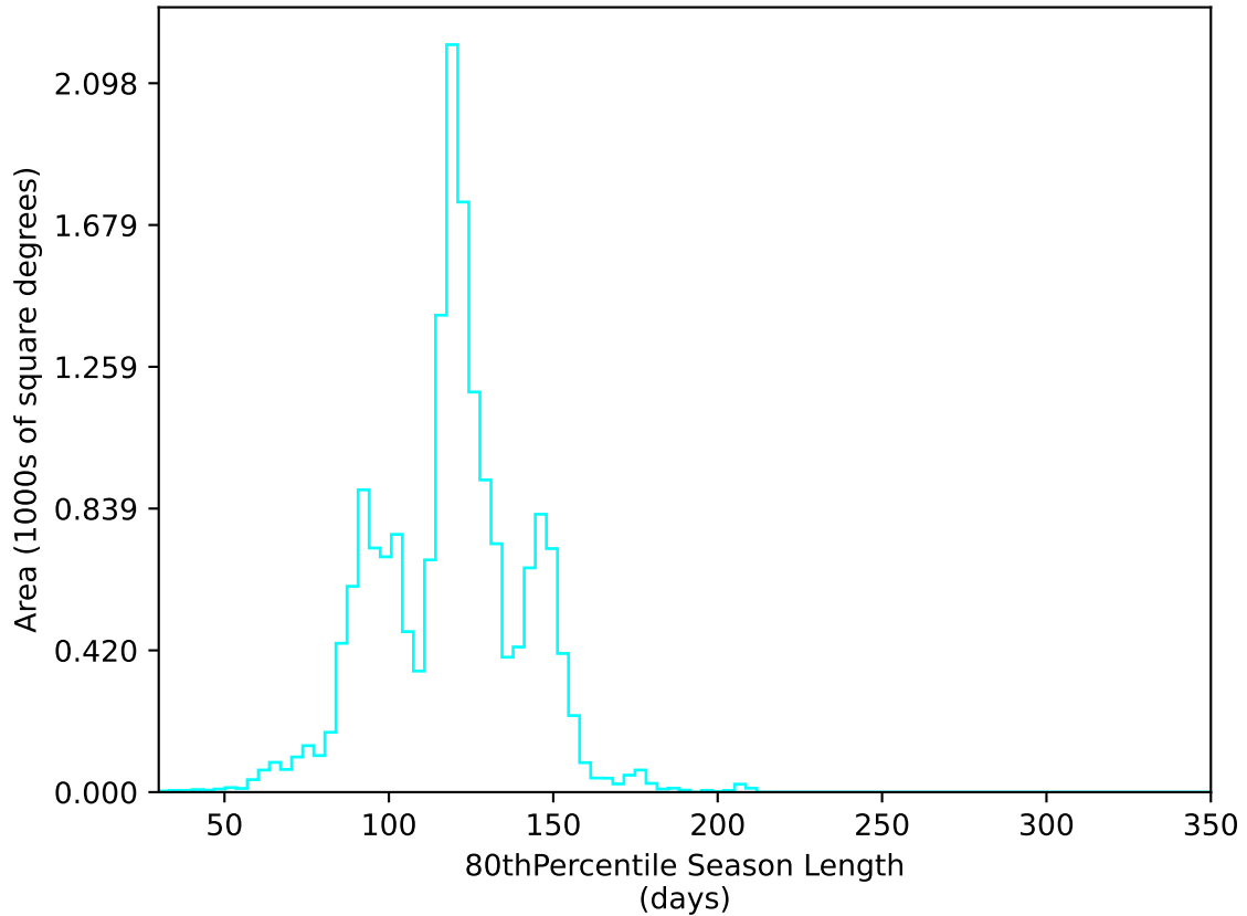
internal_u_expt30_nscale0.9v3.4_10yrs WFD u band: 80thPercentile Season Length
