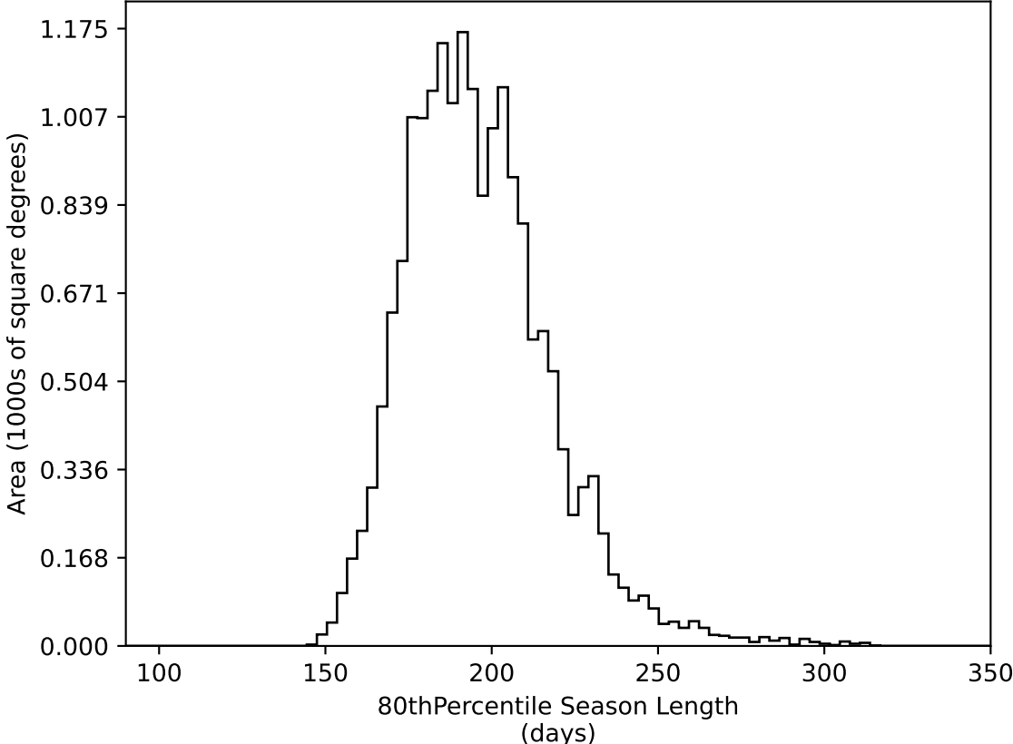
internal_u_expt30_nscale0.9v3.4_10yrs WFD all bands: 80thPercentile Season Length
