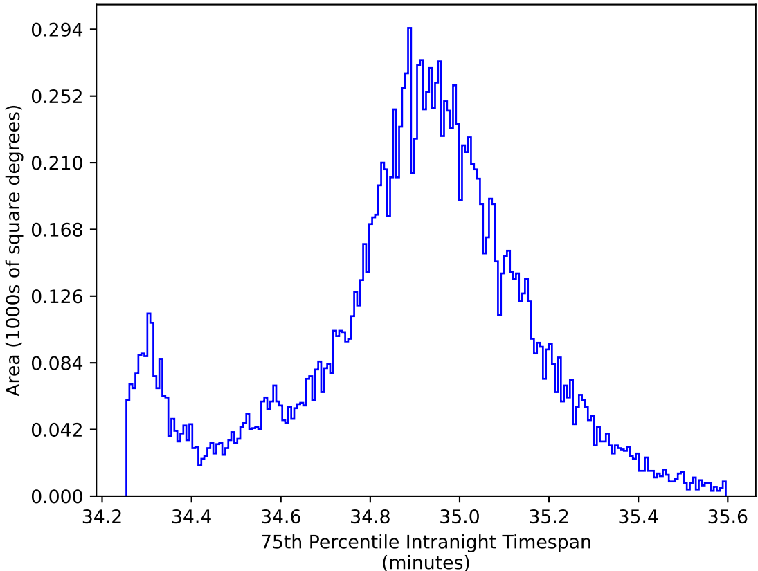
internal_u_expt30_nscale0.9v3.4_10yrs WFD: 75th Percentile Intranight Timespan
