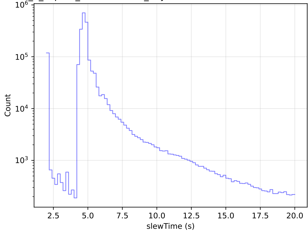
internal_u_expt30_nscale0.9v3.4_10yrs All visits: Zoom Slew Time Histogram
