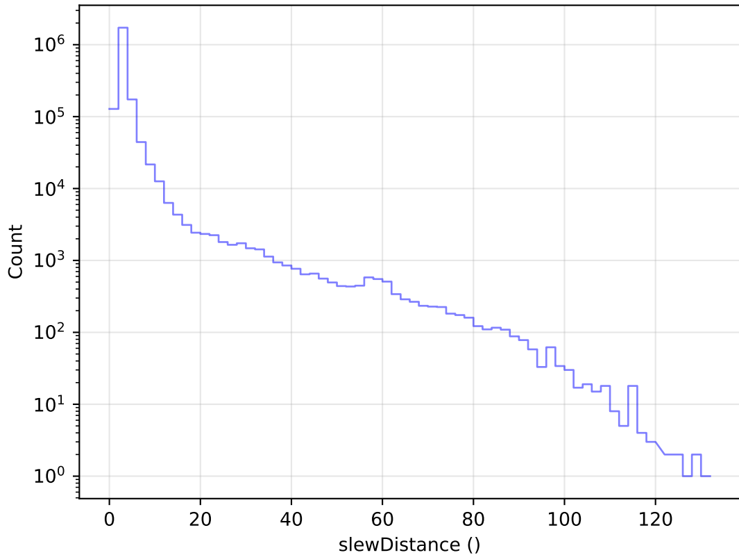
internal_u_expt30_nscale0.9v3.4_10yrs All visits: Slew Distance Histogram
