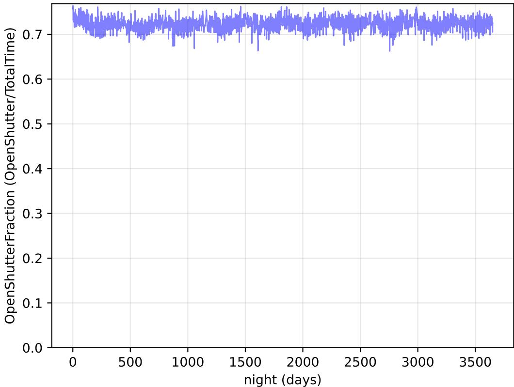
internal_u_expt30_nscale0.9v3.4_10yrs : OpenShutterFraction
