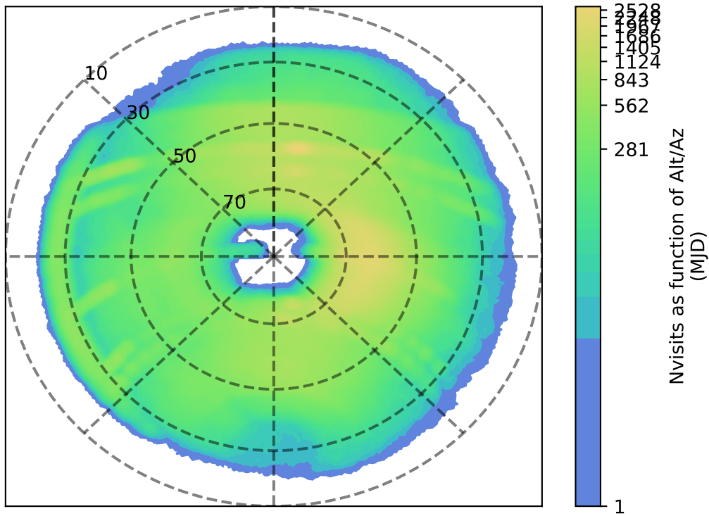
internal_u_expt30_nscale0.9v3.4_10yrs r: Nvisits as function of Alt/Az
