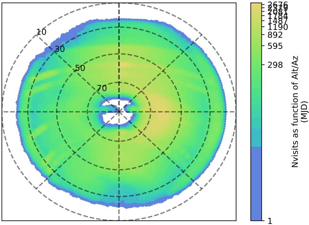
internal_u_expt30_nscale0.9v3.4_10yrs i: Nvisits as function of Alt/Az
