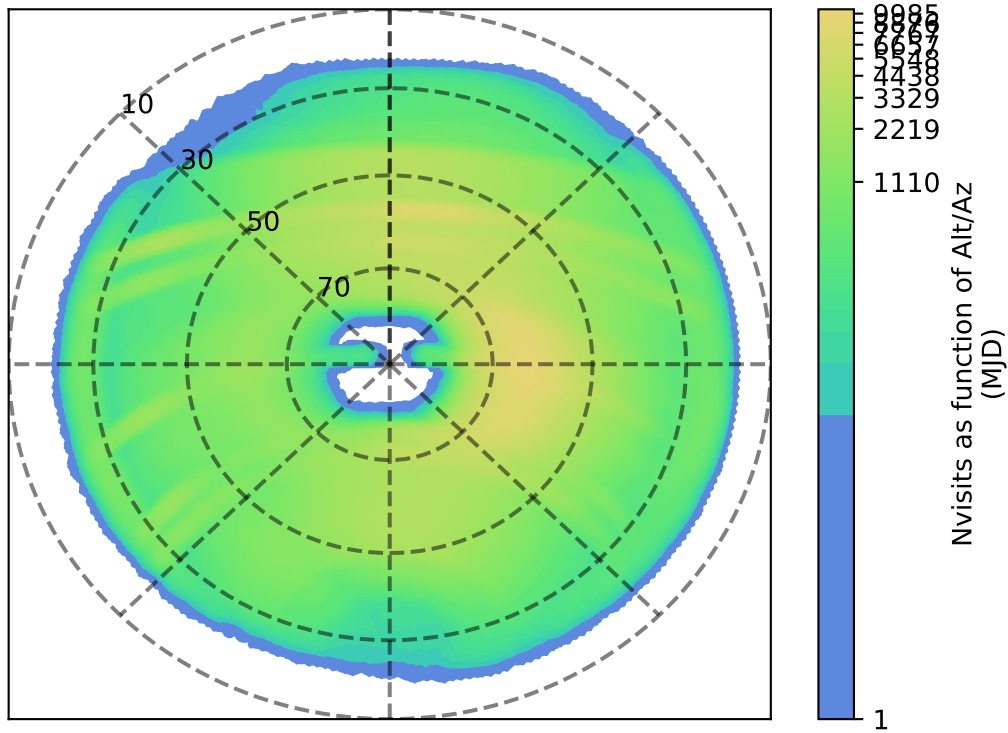
internal_u_expt30_nscale0.9v3.4_10yrs : Nvisits as function of Alt/Az
