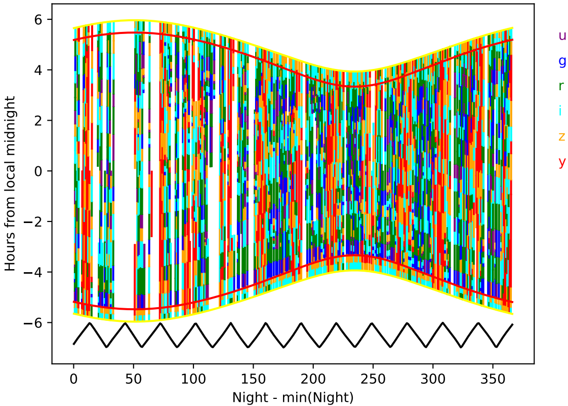
internal_u_expt30_nscale0.9v3.4_10yrs year 8-9: Hourglass
