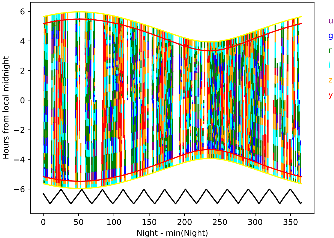
internal_u_expt30_nscale0.9v3.4_10yrs year 7-8: Hourglass
