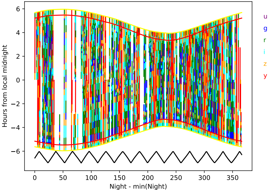
internal_u_expt30_nscale0.9v3.4_10yrs year 3-4: Hourglass
