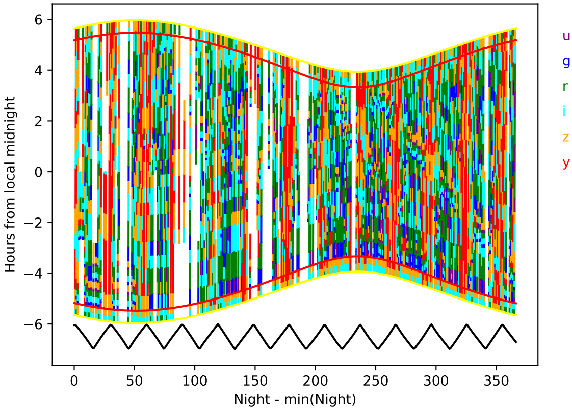
internal_u_expt30_nscale0.9v3.4_10yrs year 1-2: Hourglass
