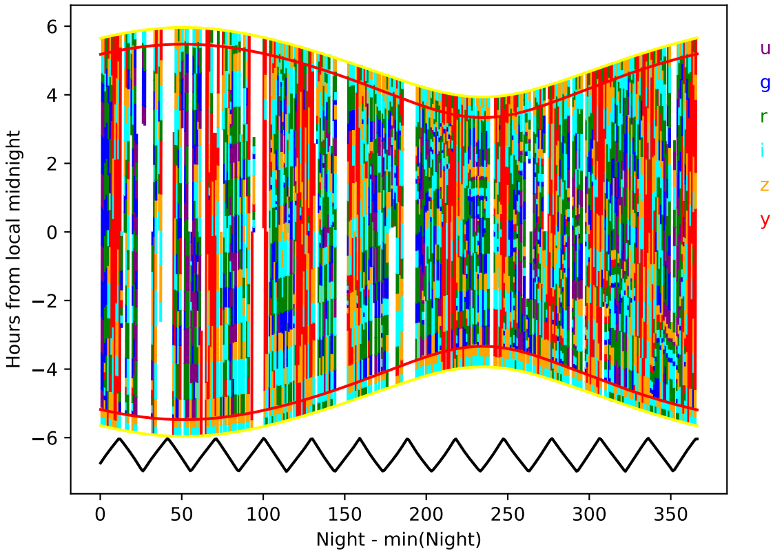
internal_u_expt30_nscale0.9v3.4_10yrs year 0-1: Hourglass
